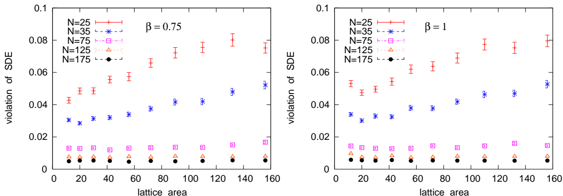
Figure 2: The convergence towards the validity of the Schwinger-Dyson equations as N increases at fixed \beta = 0.75 (on the left) and \beta = 1 (on the right). The y -axis is the absolute value of the deviation between the two sides of the specific Schwinger-Dyson equation illustrated in figure 1. The x -axis corresponds to the lattice area of the contour C , which has a rectangular shape of the form I \times (I + 1) . These equations are well approximated as N reaches \mathcal{O}(100) .
