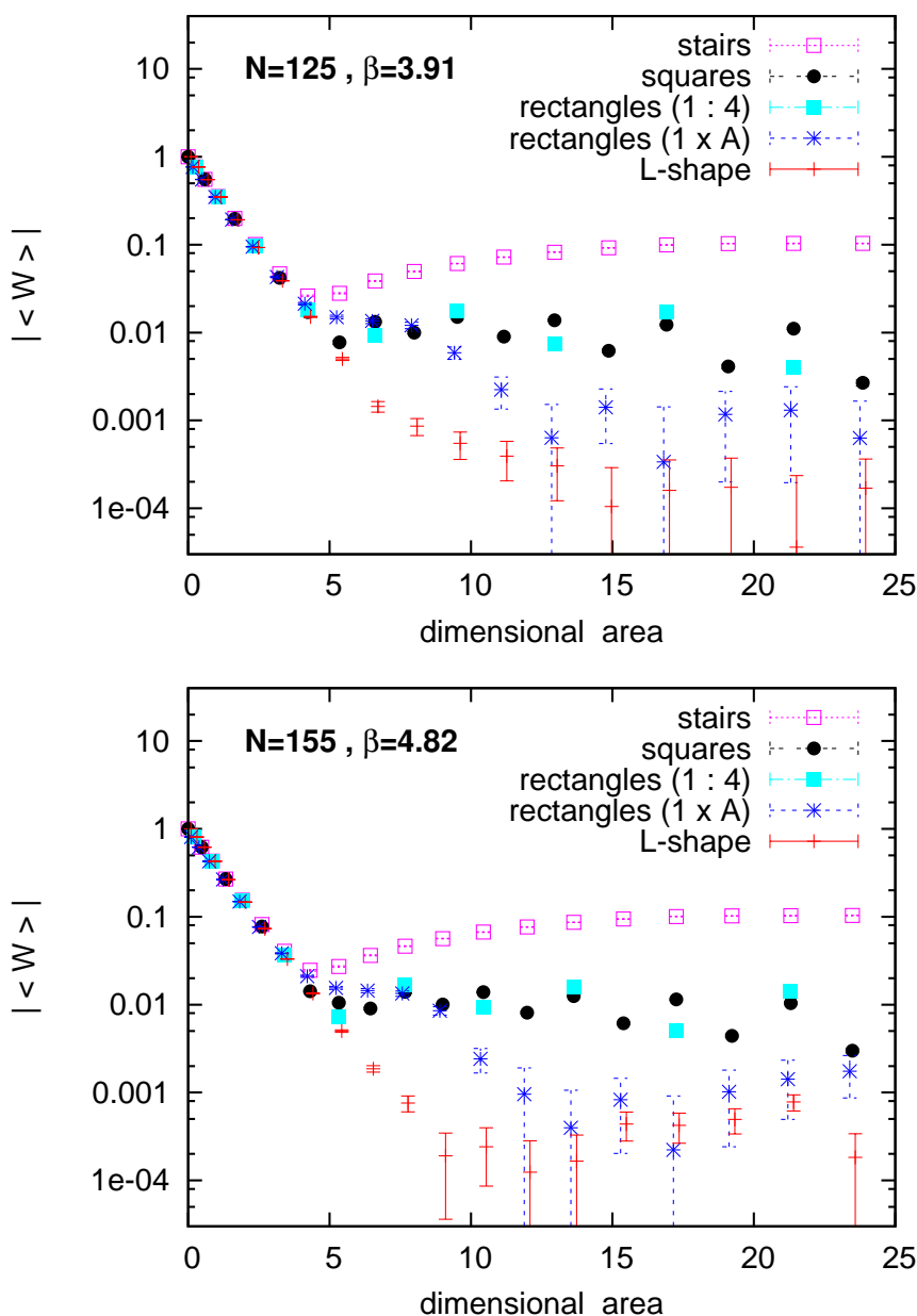
Figure 8: The analogous plots to figure 7, but now at \theta = 2.63 . Again the results clearly confirm a shape dependence beyond the area law regime, which is stable as we increase N towards the DSL.
