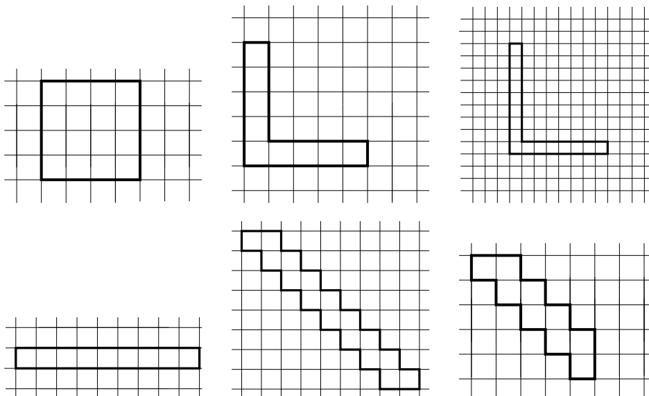
Figure 3: An illustration of the different Wilson loops that we considered. Their contours are all polygonal, without multiple-intersections. They are squares, L-shapes (with legs of width 1 lattice spacing and equal length, or lengths deviating by 1 if the area A is even), maximally anisotropic rectangles and stairs (again in two variants, depending whether A is even or odd).
