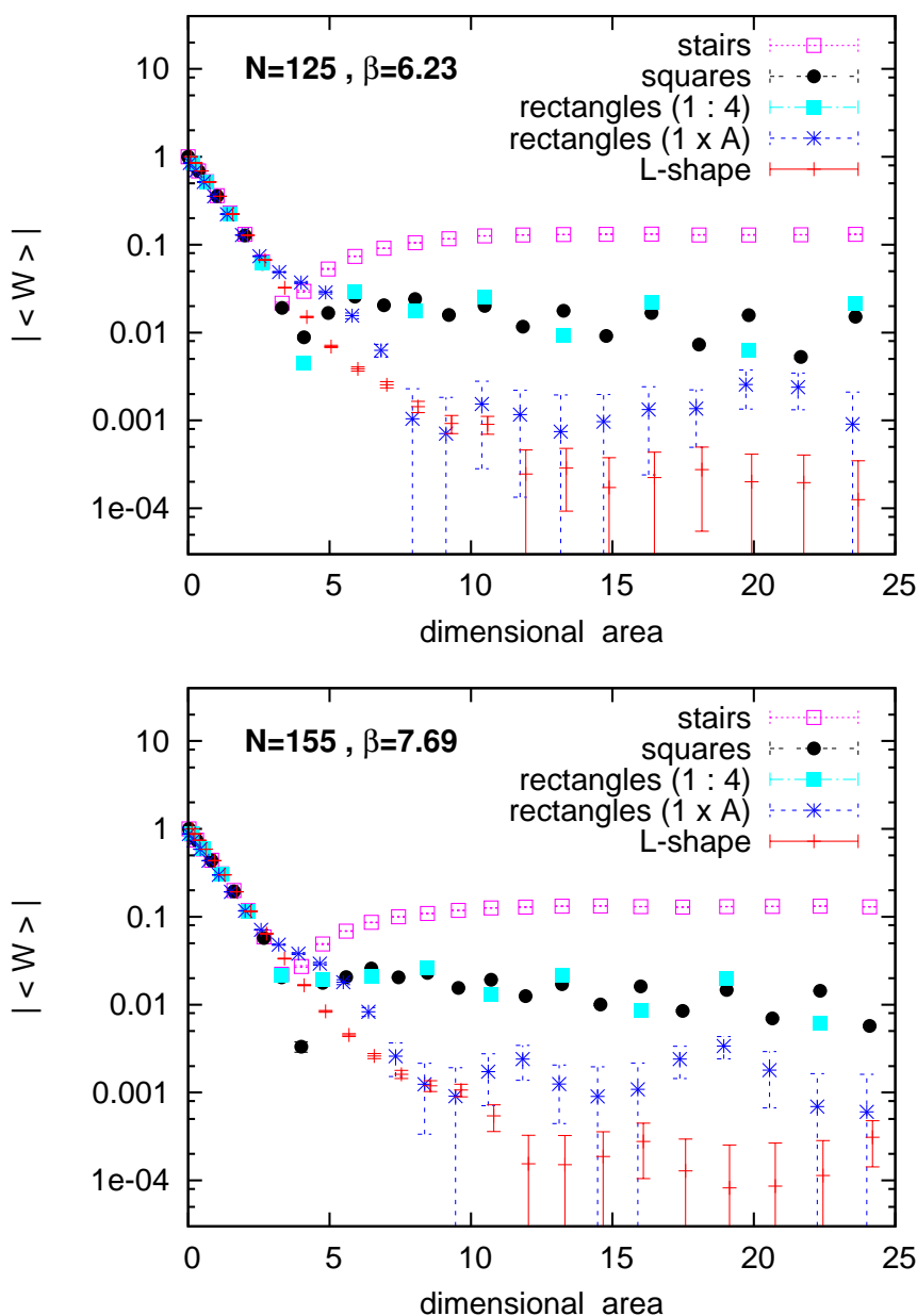
Figure 7: The absolute values of various Wilson loops at a fixed non-commutativity parameter \theta = 1.63 . On top we show results at N = 125 and below at N = 155 . As we increase N the dimensional volume grows and the lattice spacing shrinks, so that we approach simultaneously the limits to the continuum and to infinite volume (UV and IR limit). The striking similarity of these plots confirms that DSL convergence is reached. The results show a clear shape dependence beyond the area law regime, and therefore the breaking of APD symmetry.
