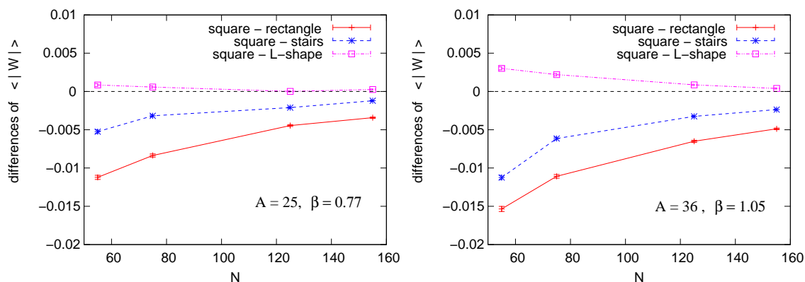
Figure 5: An illustration of the convergence towards the APD symmetry in the planar limit. On the left we show the differences of \langle |W| \rangle for Wilson loops with lattice area A = 25 at \beta = 0.77 , so the dimensional area amounts to Aa^2 \simeq 9.81 . In the plot on the right-hand-side the parameters are A = 36 and \beta = 1.05 , which implies almost the same area, Aa^2 \simeq 9.79 . For increasing N the differences between the Wilson loops with different shapes decrease rapidly, so we are approximating well the behaviour in the planar limit.
