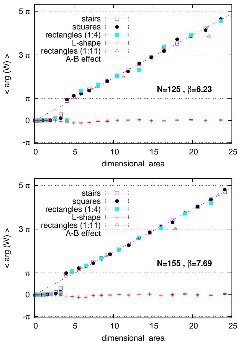
Figure 12: The phases \langle \arg(W) \rangle of various Wilson loops at \theta = 1.63 for N = 125 (on top) and N = 155 (below). The Aharonov-Bohm type behaviour in eq. (4.1) at large area holds well also for this phase for the stair loops, the squares and the rectangular loops with a fixed side ratios of 4 and of 11. On the other hand, the average phase of the L-shape loops remains very small even at large areas.
