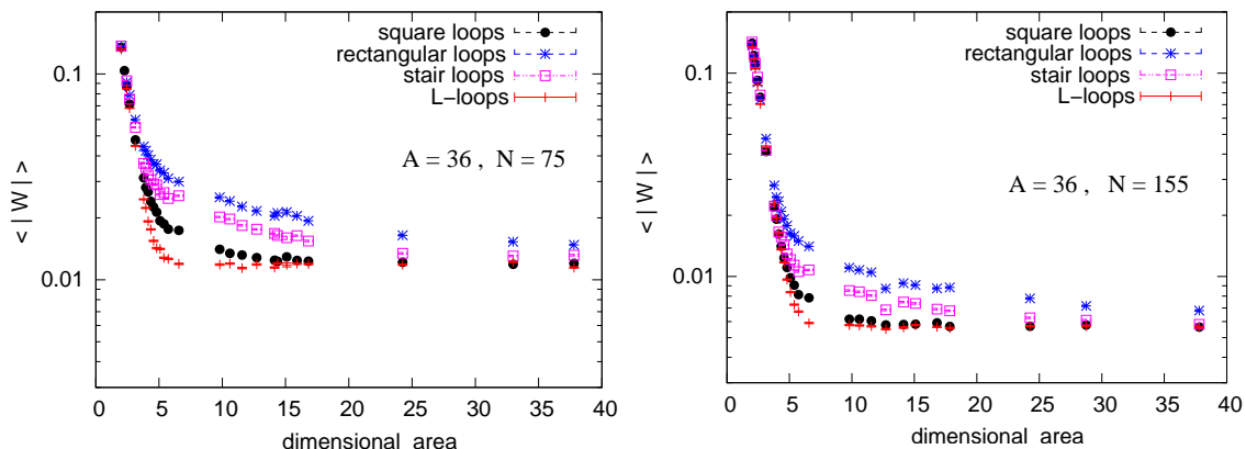
Figure 4: The absolute values of Wilson loops with different shapes and lattice area A = 36 . They are plotted against the physical area 36a^2 , which is varied by using different values of \beta . We show results for N = 75 on the left, and for N = 155 on the right. The results for different shapes coincide best at small and at larger areas, but they differ most around 36a^2 \approx 10 .
