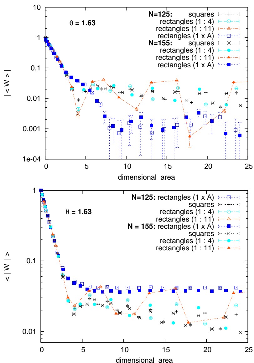
Figure 14: The decay of the absolute values |\langle W \rangle| (on top) and of \langle |W| \rangle (below) for rectangular loops at \theta = 1.63 . Beyond the area law regime, the rectangles with finite sides in the DSL (i.e. with a fixed side ratio) tend to oscillate around \approx 0.01 for |\langle W \rangle| and a somewhat larger value for \langle |W| \rangle . The amplitudes, however, depend clearly on the side ratio, which shows the SL(2, R) symmetry breaking. This is most evident for the rectangles with side ratio 11 (their data are connected by a line to guide the eye).
