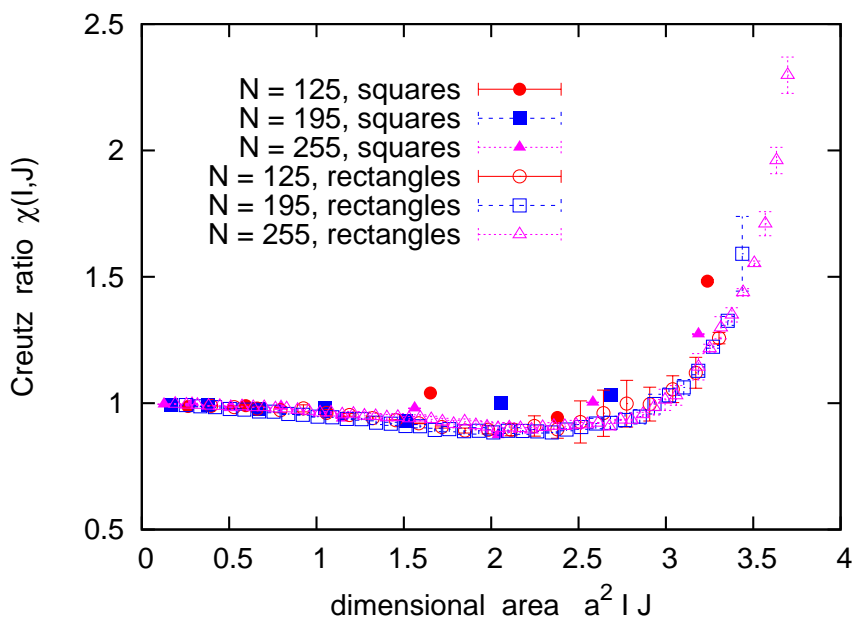
Figure 6: The Creutz ratio \chi(I, J) for Wilson loops with small areas, up to the transition at the end of the area law regime. The parameter sets are (N, \beta) = (125, 3.91) , (195, 6.09) and (255, 7.97) , which all corresponds to \theta \approx 2.6 , so we are approaching a DSL. For both shapes, i.e. for \chi(I, I) (squares) and for \chi(2, J) (rectangles), we observe stable Creutz ratios in the DSL. At small area the string tension takes the same value as in the planar limit. At moderate area the results from square shaped and from extremely anisotropic rectangles begin to differ a little.
