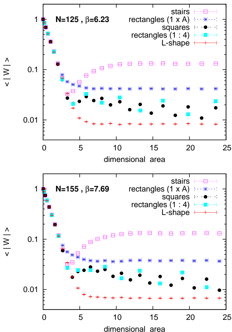
Figure 10: The expectation values \langle |W| \rangle for various Wilson loops at a fixed non-commutativity parameter \theta = 1.63 . On top we show results at N = 125 and below at N = 155 . The striking similarity of these plots confirms that DSL convergence is reached. The results reveal a clear shape dependence beyond the area law regime also for this observable.
