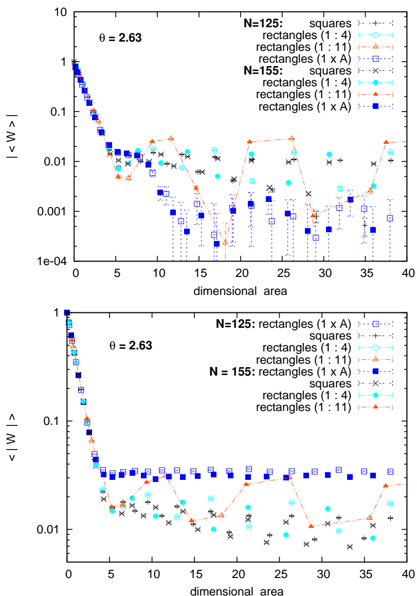
Figure 15: The analogous plots to figure 14, but now at \theta = 2.63 . The observed decays of the rectangular Wilson loops is very similar for both non-commutativity parameters \theta that we consider. Again the SL(2, R) symmetry breaking can be seen best from the data for rectangles with side ratio 11 (which are connected to guide the eye).
