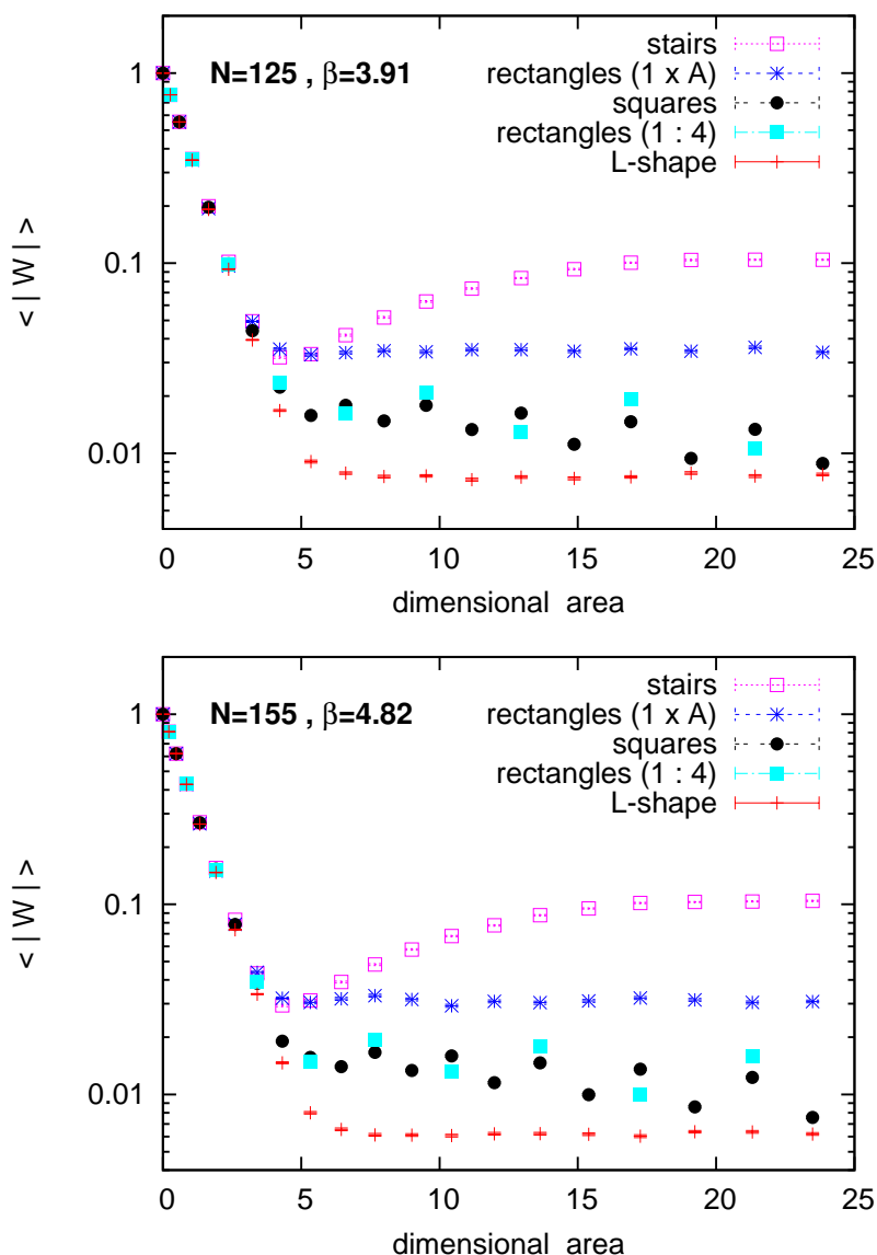
Figure 11: The analogous plots to figure 10, but now at \theta = 2.63 . The results affirm once more a shape dependence beyond the area law regime, which is stable as we increase N . In particular the differences at fixed area do not shrink as we increase N towards the DSL, in contrast to the planar limit behaviour in figure 5.
