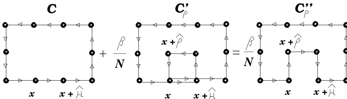
Figure 1: An example of a set of contours, which are involved in a Schwinger-Dyson equation. These equations relate the vacuum expectation values of the corresponding Wilson loops in the planar limit. They can be derived from the invariance under an infinitesimal substitution of the compact link variables on the lattice [22].
