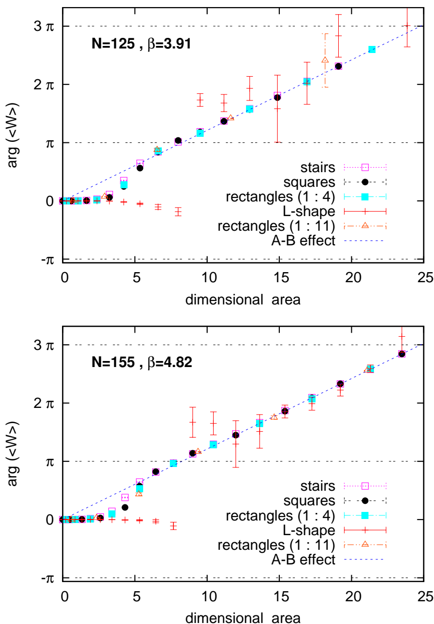
Figure 9: The phases of various Wilson loops at \theta = 2.63 for N = 125 (on top) and N = 155 (below). The Aharonov-Bohm type behaviour in eq. (4.1) at large area is very well confirmed for the shapes shown here. They include results for rectangular loops with a fixed ratio of 4 and a ratio of 11 between the side lengths, so that its shape is invariant on the way to the DSL. The L-shape, on the other hand, becomes infinitesimally thin in this limit. Its phase follows eq. (4.1) with some fluctuations.
