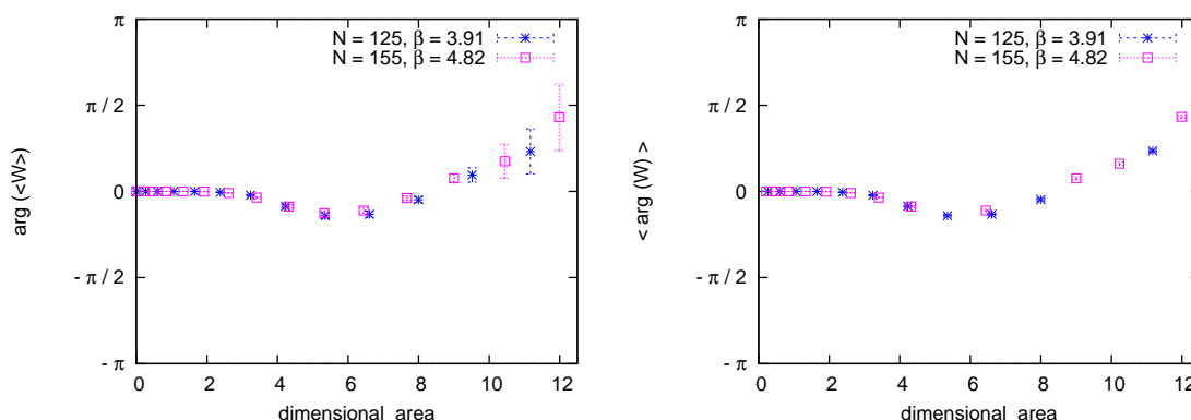
Figure 13: The phases of narrow rectangles with the shape 1 \times A at \theta = 2.62 . We show the phase of \langle W \rangle (on the left) and the expectation value of \arg(W) (on the right). Their values are very similar, but these phases are not related to eq. (4.1). The essential observation here is that the phases practically coincide for the two sets of parameters, which confirms again that we do see the window that extrapolates to the DSL.
